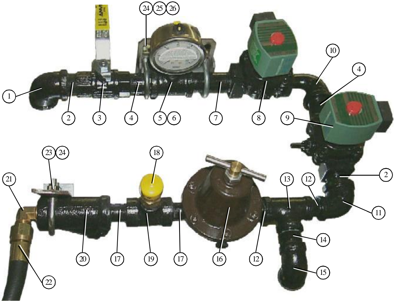
36" Fan heater LP pipe train assembly.
